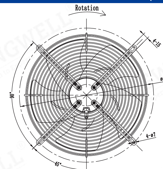
LWAD3G300ZB-5PEW-04(吹风)
