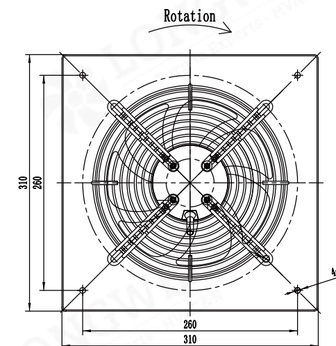
LWAD3G200ZB-7MGW-08(吹风)
