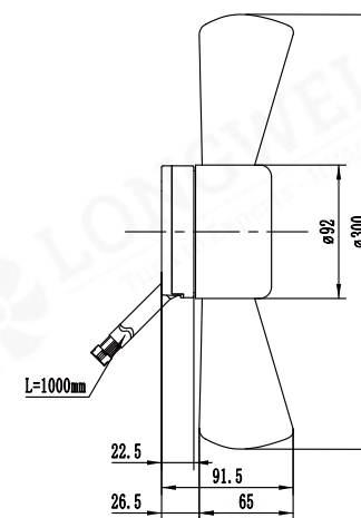
LWAD3G300ZS-5PEW-03(吸风)
