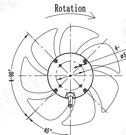
LWAD3G200ZB-7MNV-04(吹风)
