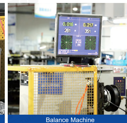
Balance Machine
