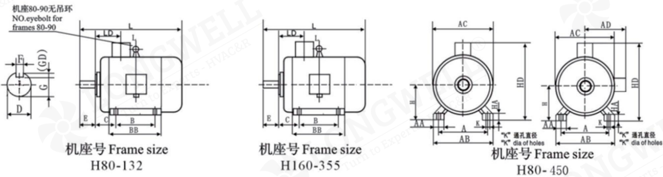
Motor with feet on frame and without flange on end shields unit: mm
