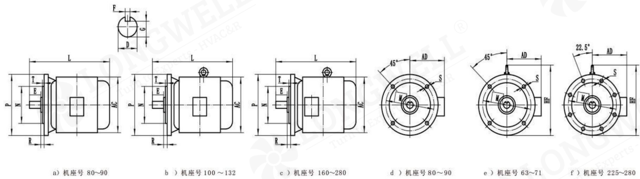
Electric motor with a base without feet and a flange (with through-hole) on the end cover unit: mm
