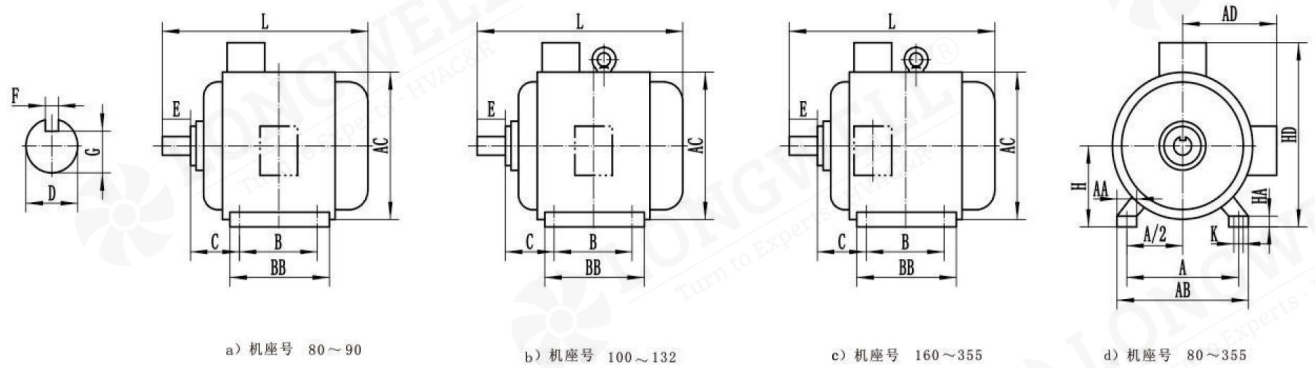
Electric motor with base with feet and no flange on the end cover unit: mm
