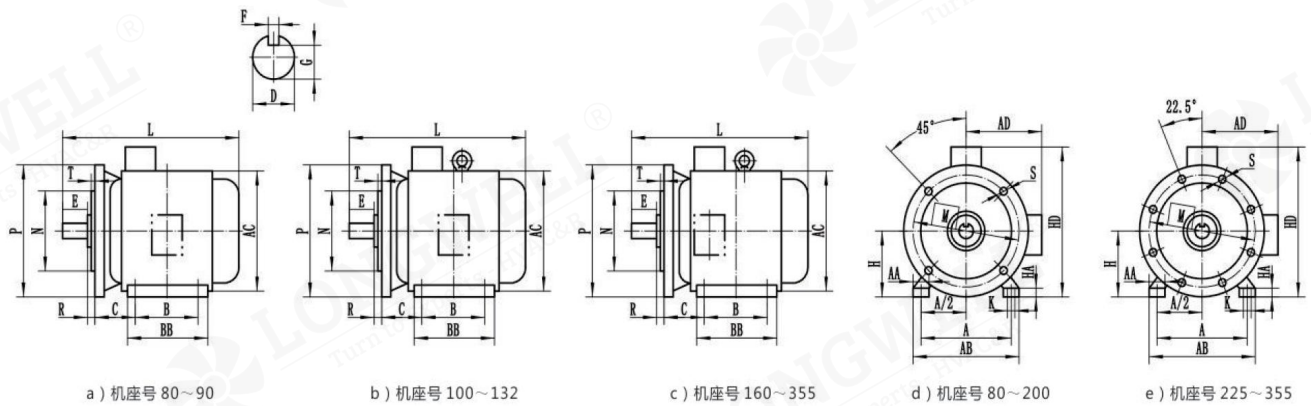
Electric motor with base and flange (with through-hole) on end cover unit: mm
