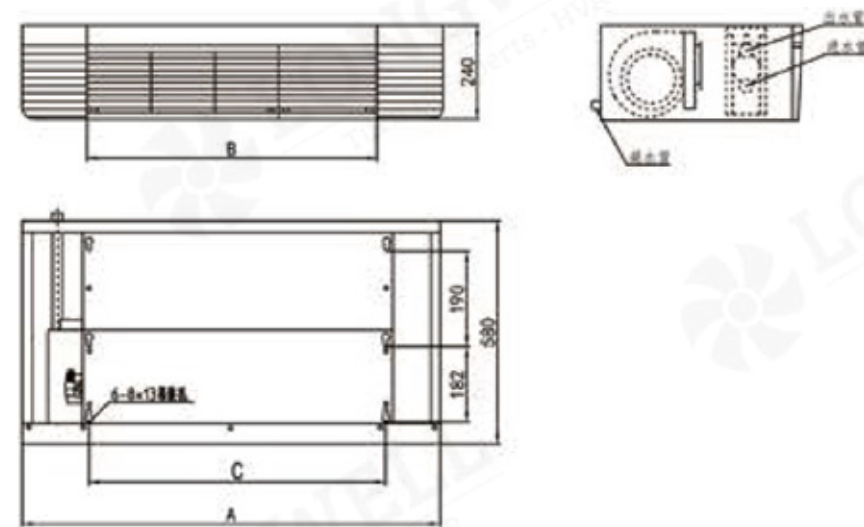
Horizontal Exposed Series Dimensional Diagram
