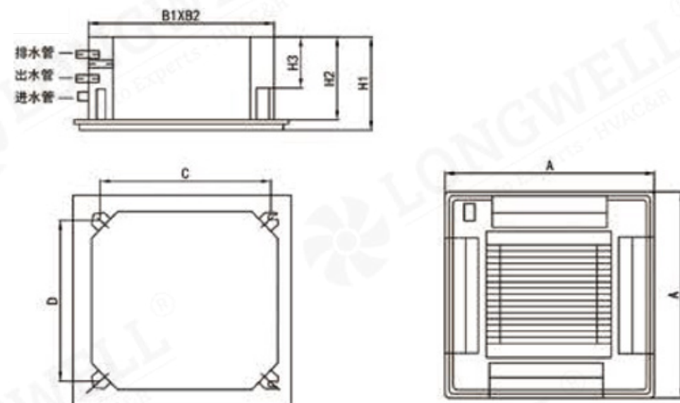
Cassette Exposed Series Dimensional Diagram
