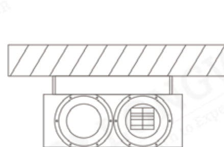
Normal horizontal installation (access door cannot face down)
