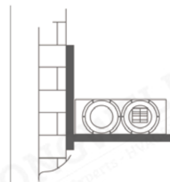
Triangular bracket auxiliary installation
