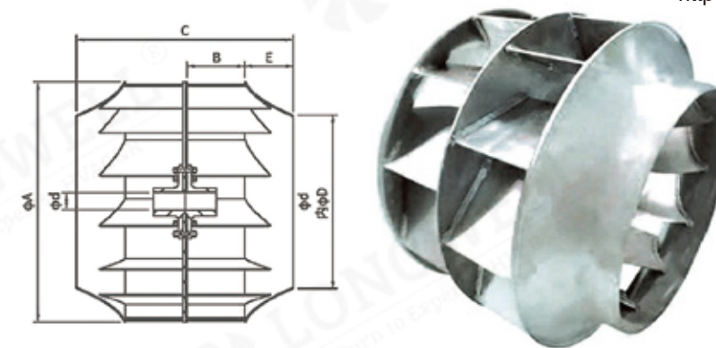
Dual Inlet Backward Impellers
